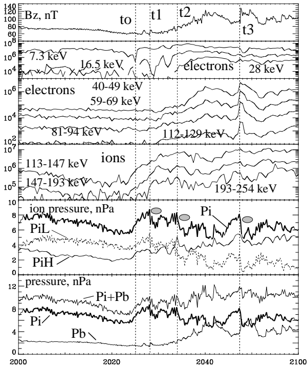
Fig.3. Substorm B. Shown in the same format as Fig. 1.
